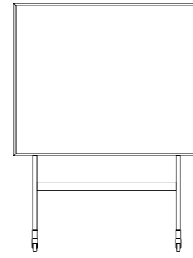
1508 x 1960 x 500
